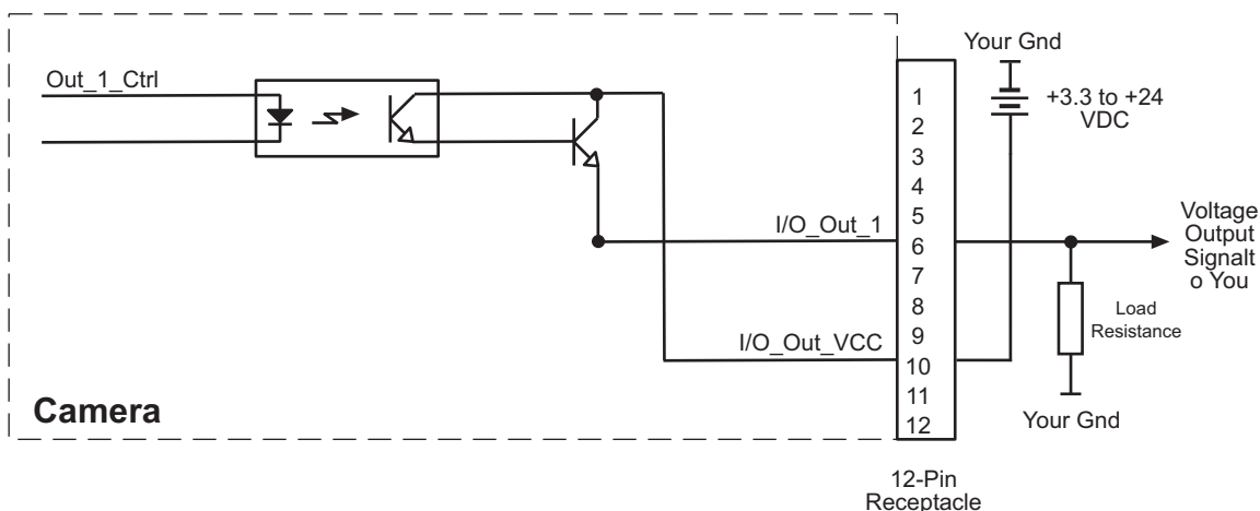
Fig. 24: Typical Voltage Output Circuit
