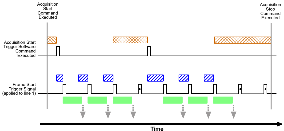
Fig. 43: Use Case 4 - Acquisition Start Trigger On and Frame Start Trigger On
