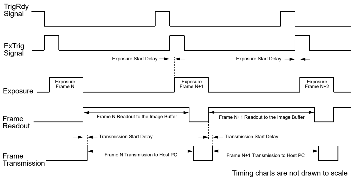
Fig. 49: Exposure Start Controlled with an ExTrig Signal
