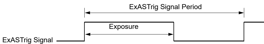
Fig. 38: Trigger Width Exposure with Rising Edge Triggering
