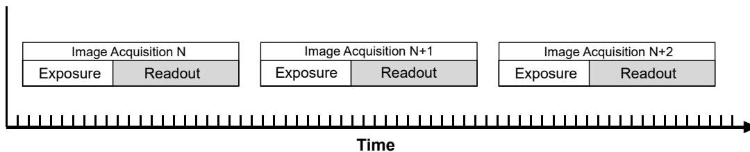
Fig. 44: Non-overlapped Exposure
