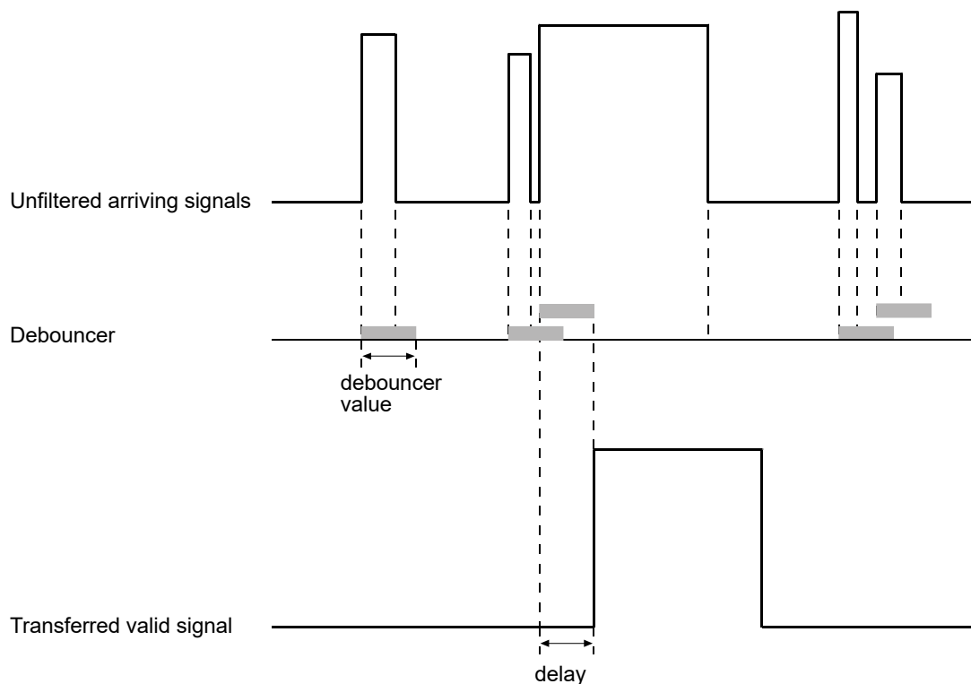
Fig. 71: Filtering of Input Signals by the Debouncer
