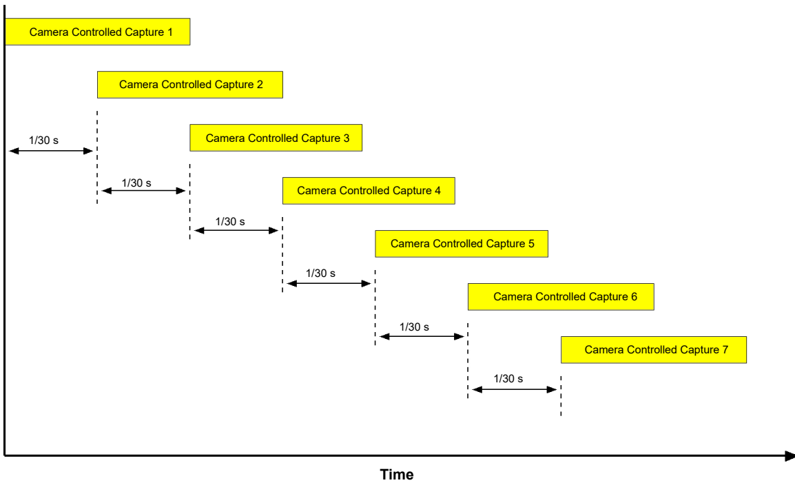
Fig. 15: Normal Image Capture
