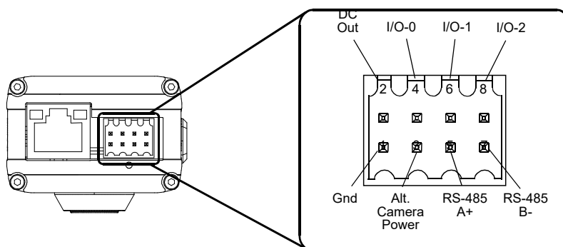
Fig. 9: Terminal Connector Pin Numbering
