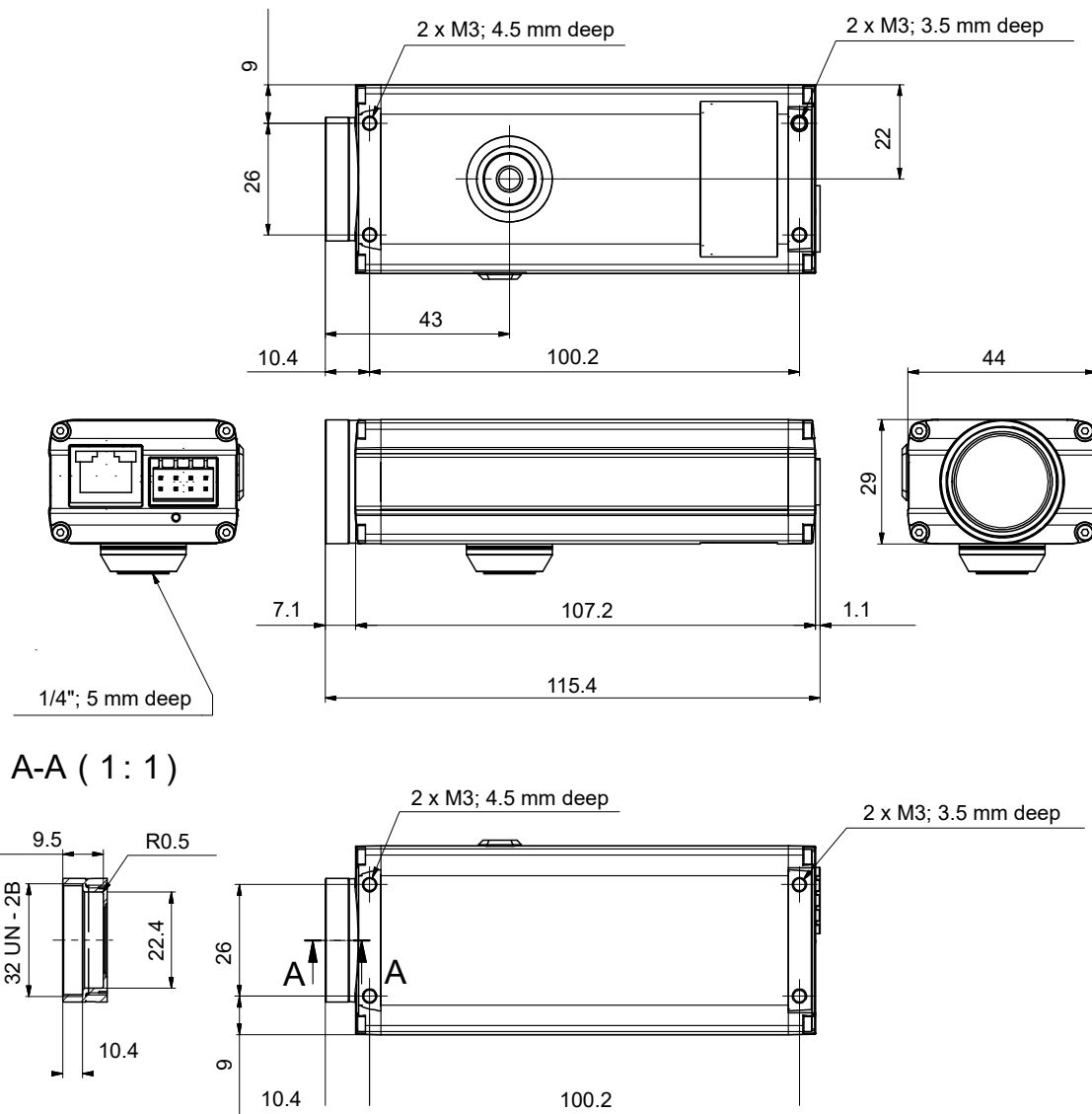
Fig. 18: C-Mount Camera Dimensions (in mm unless otherwise stated)
