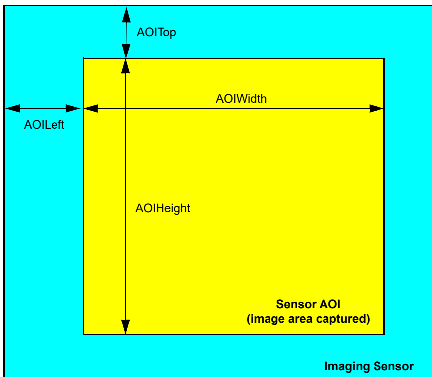
Fig. 3: Sensor AOI
