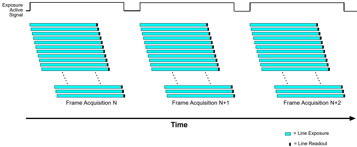
Fig. 8: Exposure Active Signal
