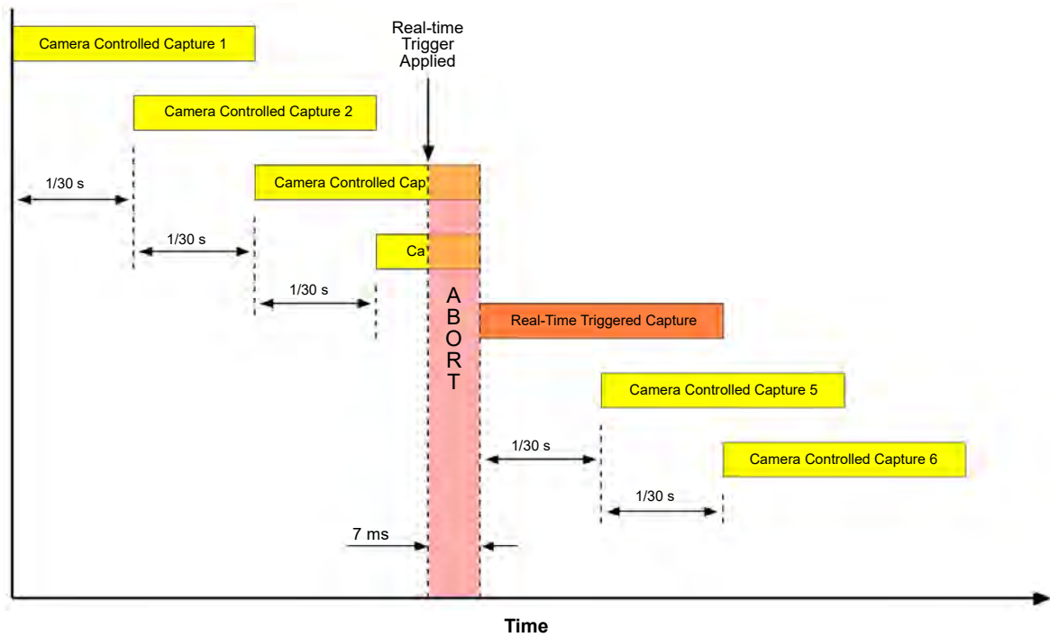
Fig. 16: Real-Time Trigger Image Capture
