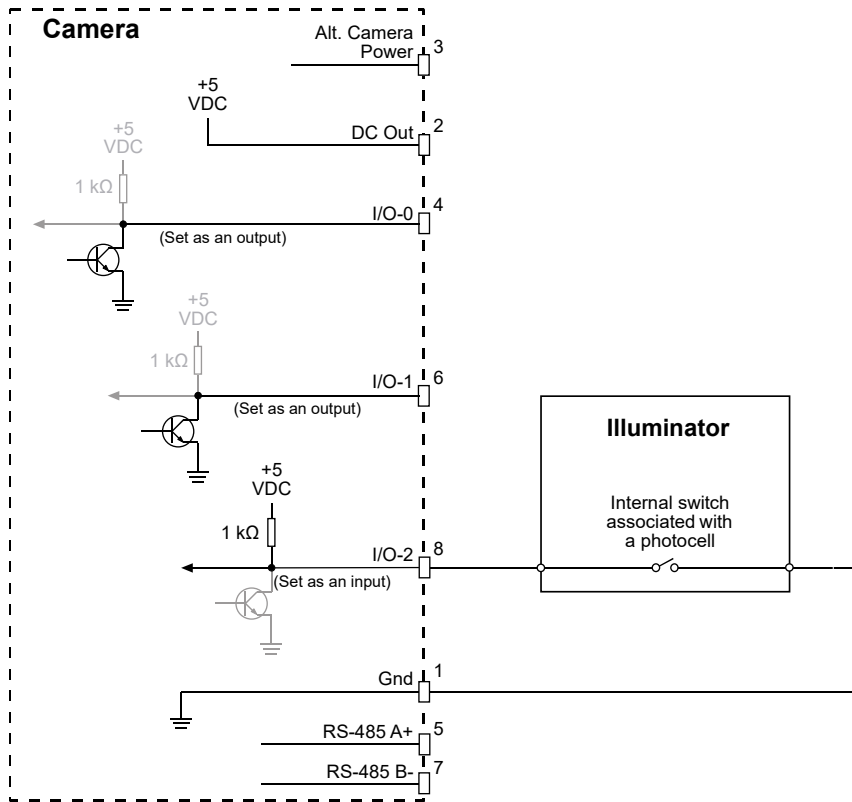
Fig. 13: Input Used to Control IR-Cut Filter Position
