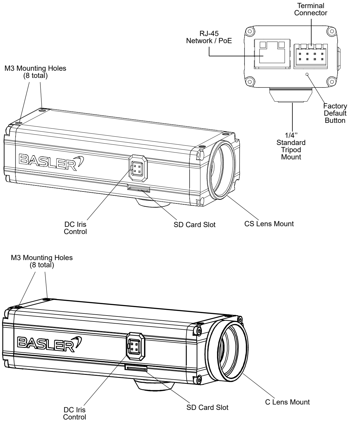
Fig. 1: Camera Connections for C-Mount and CS-Mount Camera Models
