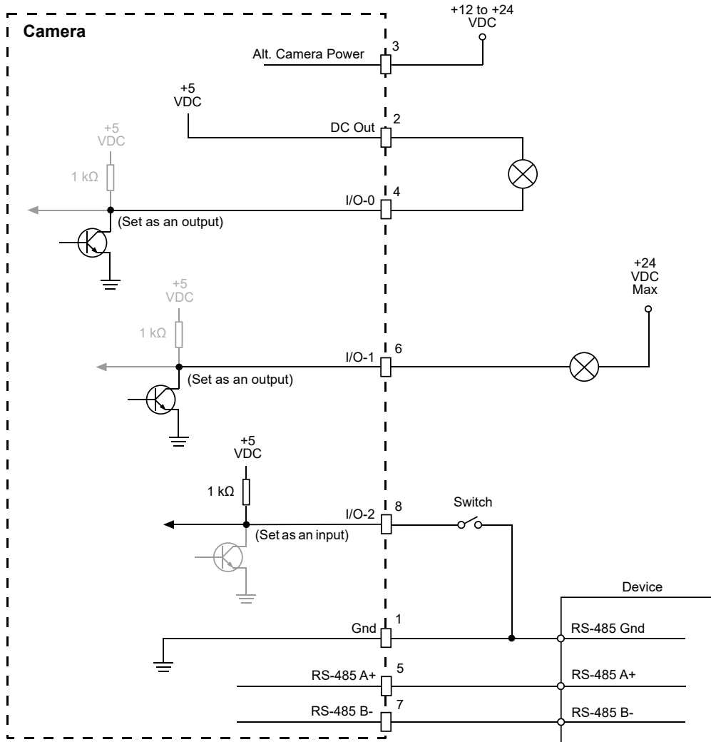
Fig. 11: I/O Schematic, Variant 1 (Input Port Connected to Ground via Switch)
