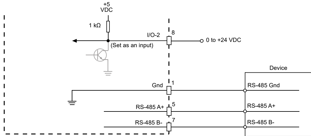
Fig. 12: I/O Schematic, Variant 2 (Input Port Connected to Input Voltage)
