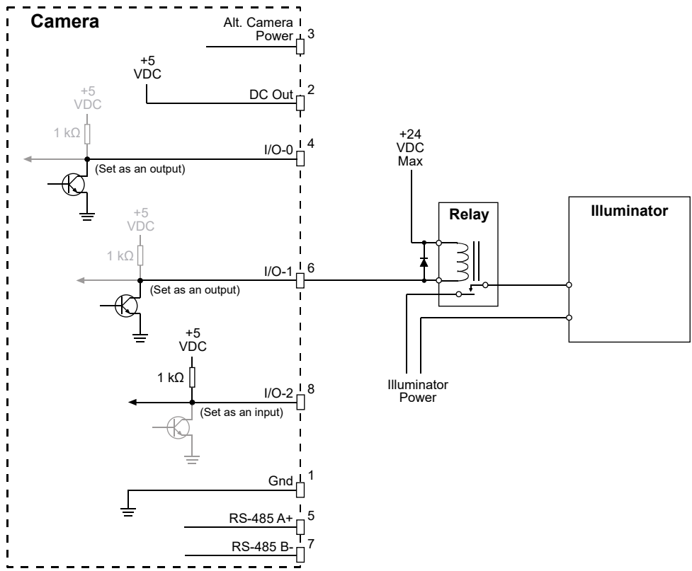
Fig. 14: Output Used to Apply Device Power
