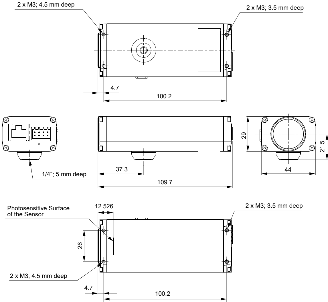
Fig. 17: CS-Mount Camera Dimensions (in mm unless otherwise stated)
