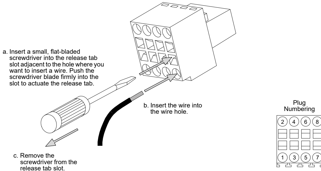
Fig. 10: Wire Insertion Method
