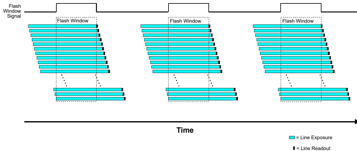
Fig. 7: Flash Window Signal
