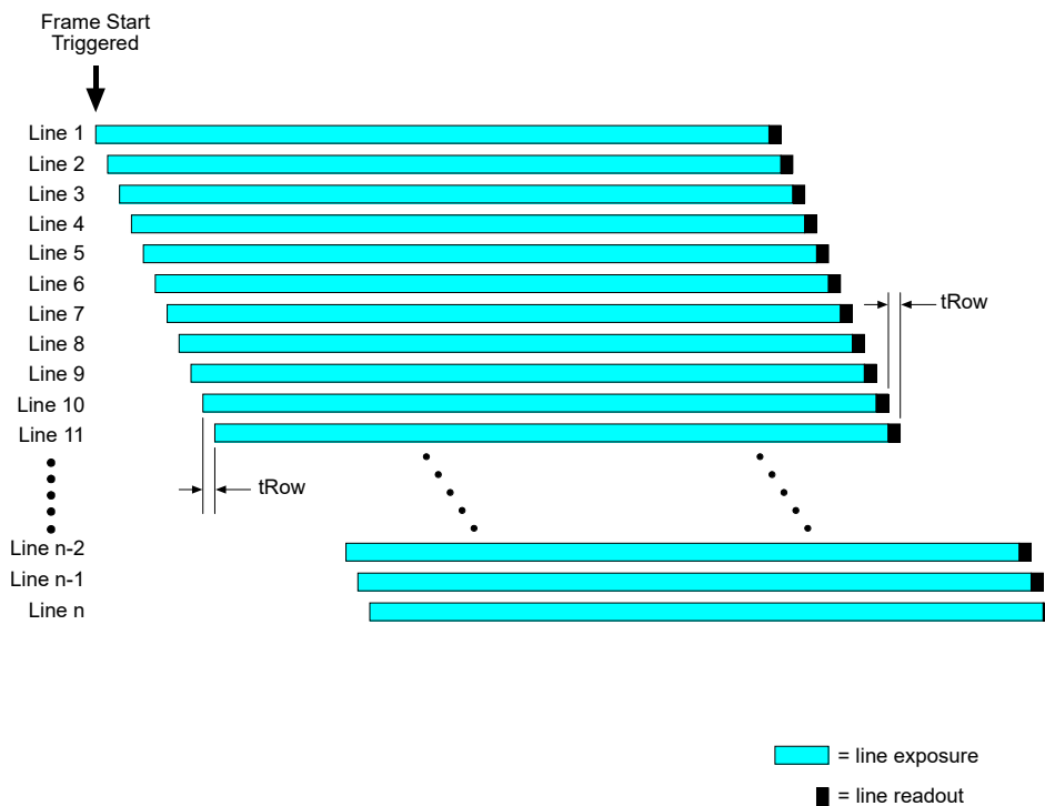
Fig. 5: Rolling Shutter
