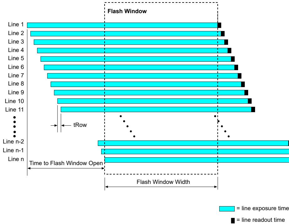
Fig. 6: Flash Window
