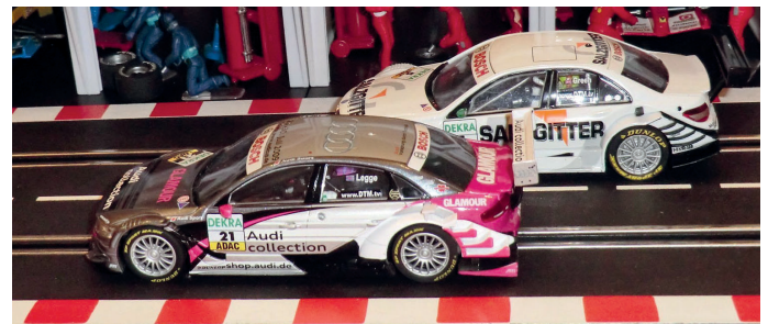
Fig. 8: Global shutter at standard resolution
